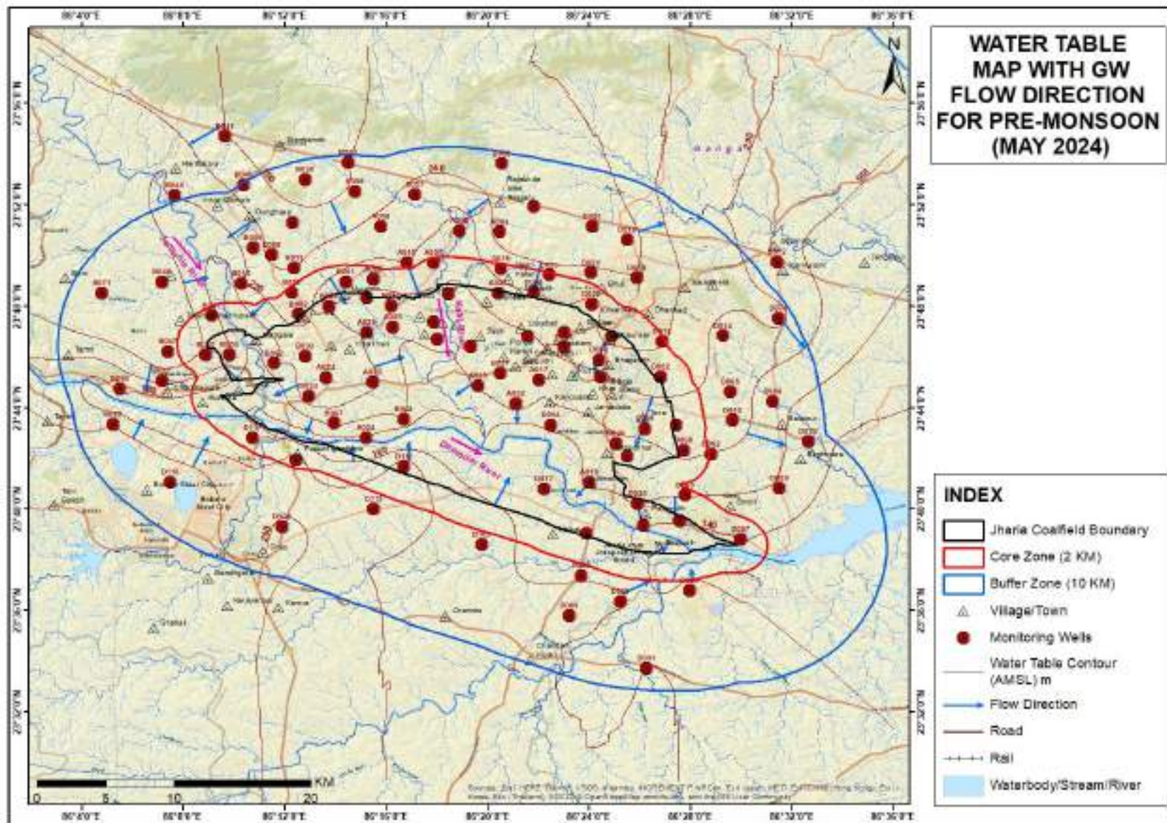
Plate- IVA: Water table Contour Map of JCF, Pre Monsoon (May'24)
