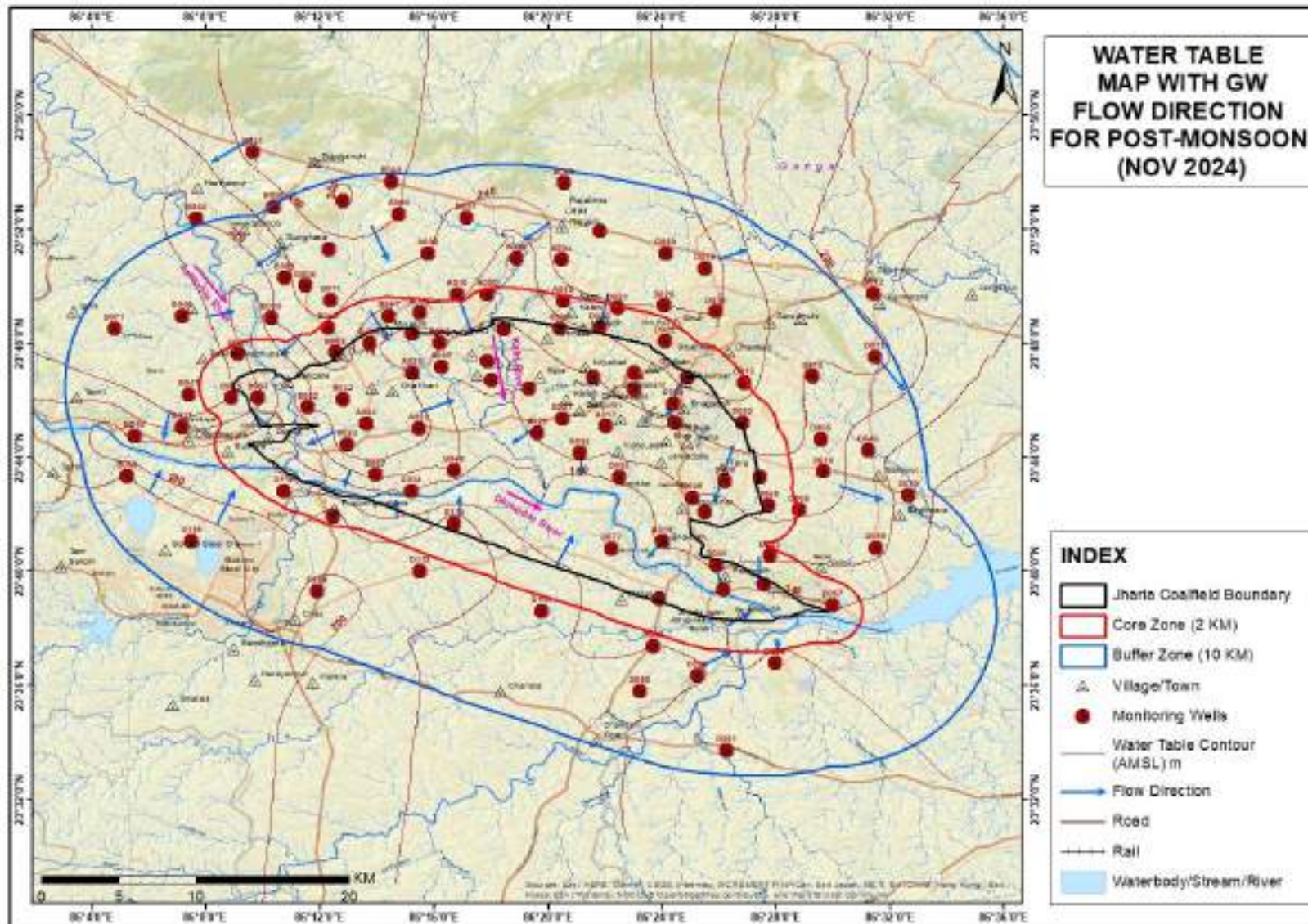
Plate- IVB: Water table Contour Map of JCF, Post Monsoon (Nov'24)
