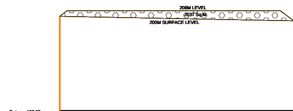
LONGITUDINAL SECTION ALONG- A5 - A6 OF PROPOSED OB DUMP NO.- 4
